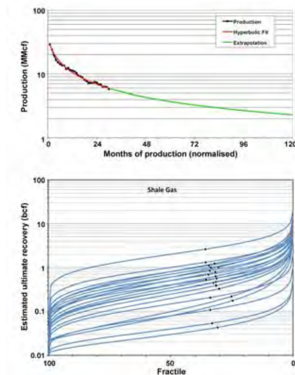
Figure 4. A typical gas production curve (upper) and the probability distribution of estimated ultimate gas recovery (lower) based on actual North American shale gas plays, after Gautier (2012). Each curve in the lower plot is derived from the aggregation of estimated ultimate recovery values for all wells within a given shale gas play. The USGS assessment method uses productivity models based on such production data to estimate the technically recoverable resource volumes
