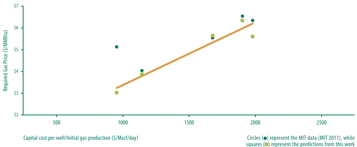
Figure A.3.3: Plot of required gas price versus capital intensity for both the MIT study and the present work
