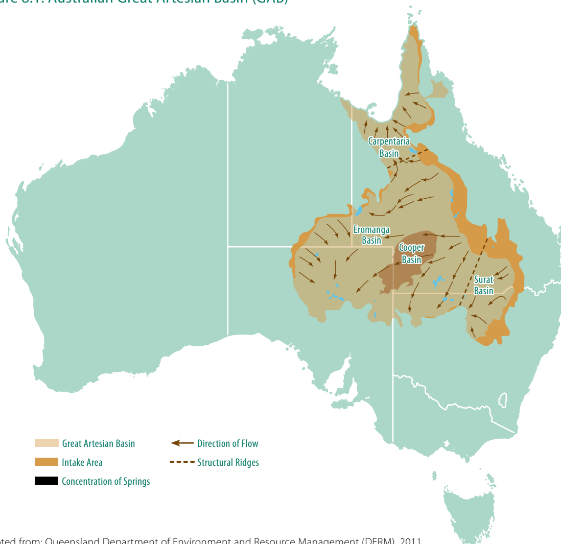
Figure 8.1: Australian Great Artesian Basin (GAB)
