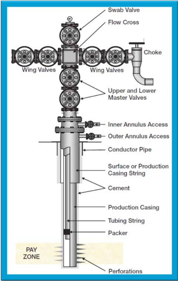
Figure 5: Hydraulic stimulation wellhead fixture example 15
