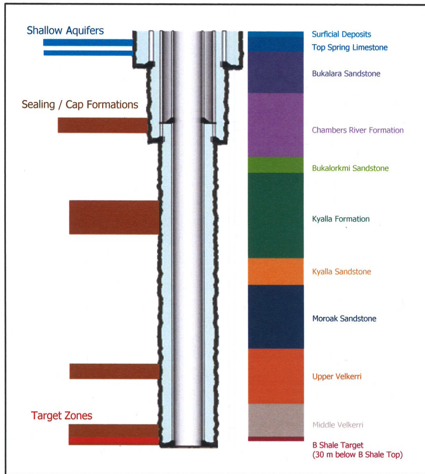
+ Conceptual well design
