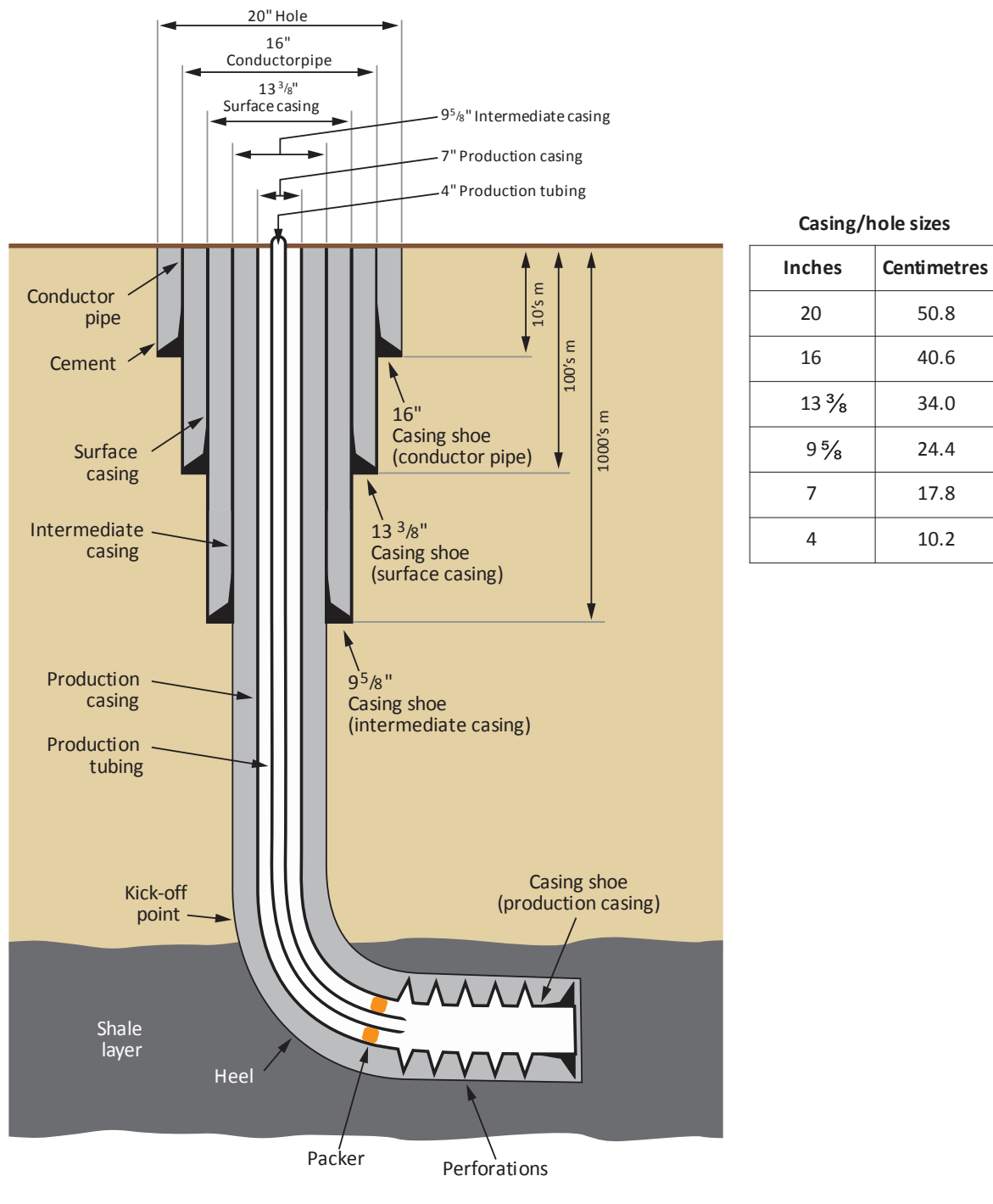
Figure 3: General layout of casing in a shale gas well. Casing sizes are specified in imperial units. Not to scale (width is significantly exaggerated).
