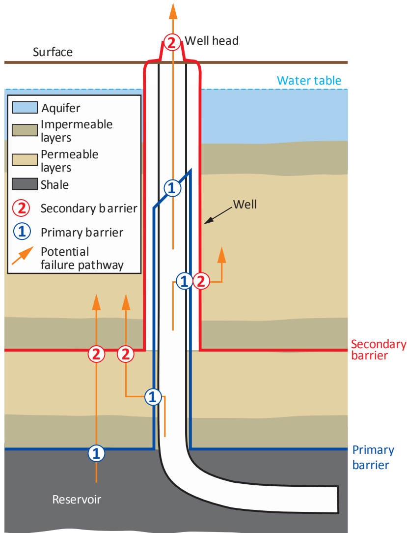
Figure 7: The two-barrier concept, showing the two barriers to various pathways for fluid flow out of the well.
