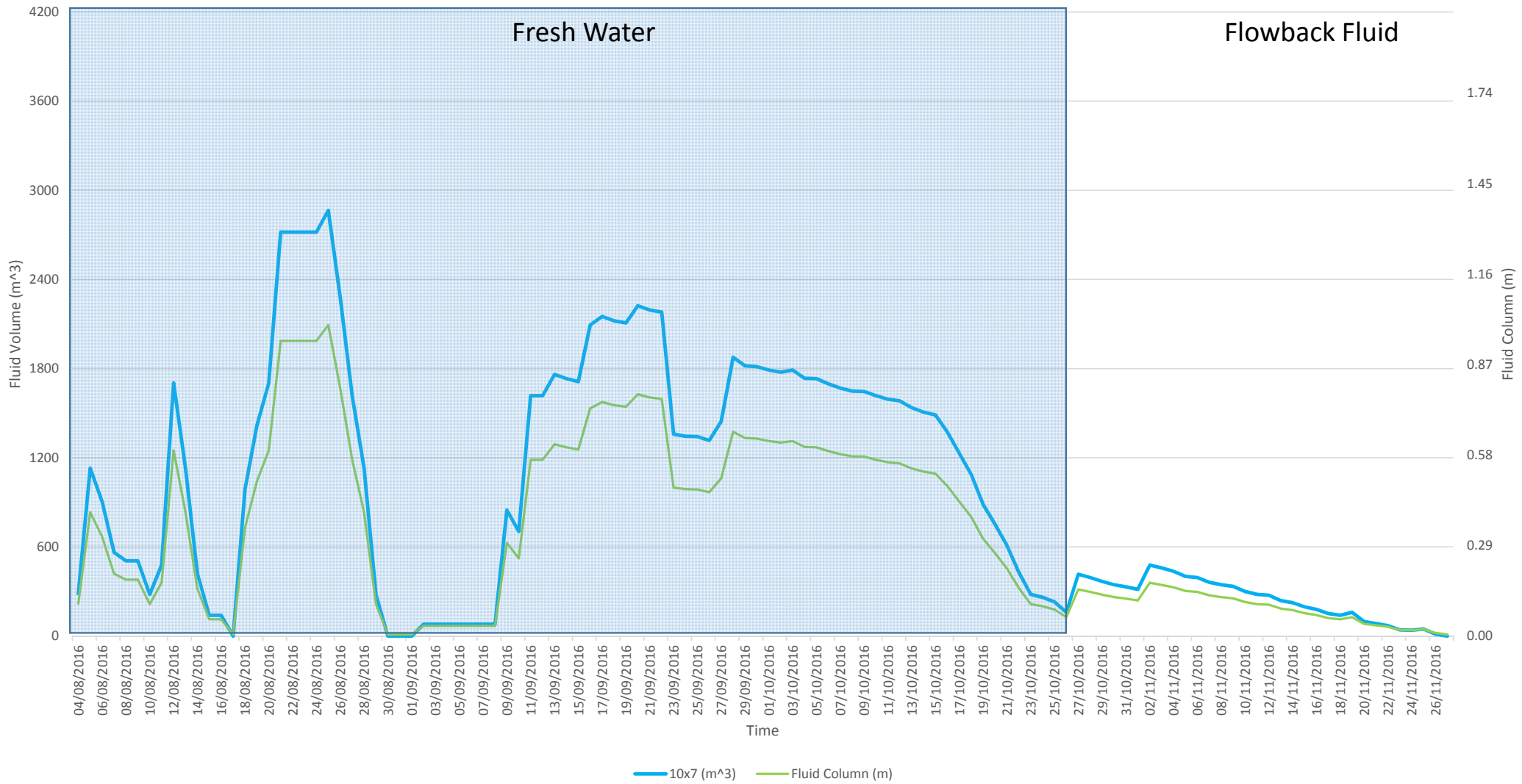
Volume and fluid column height over time Amungee NW-1 10*7 pond
