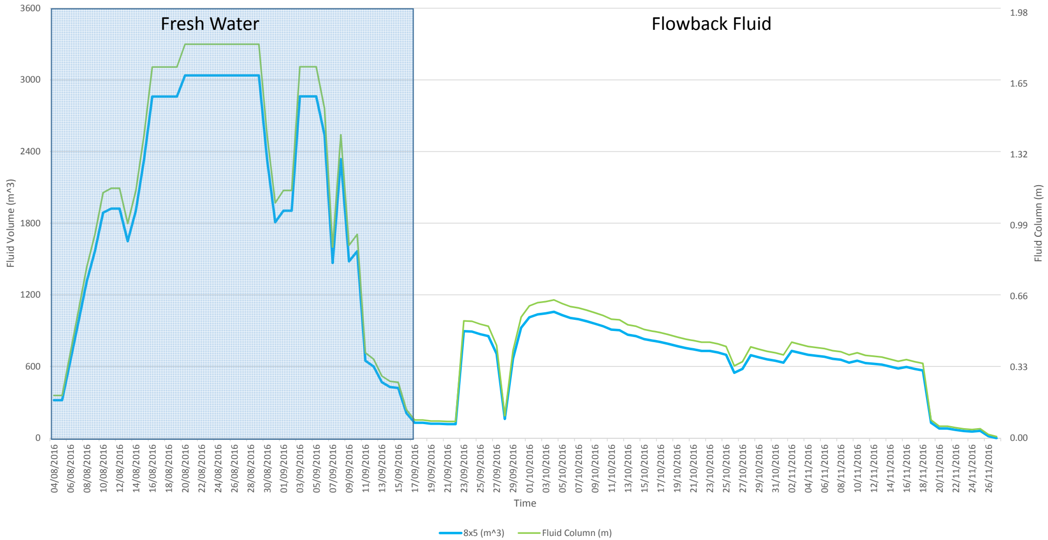
Volume and fluid column height over time Amungee NW-1 8*5 pond
