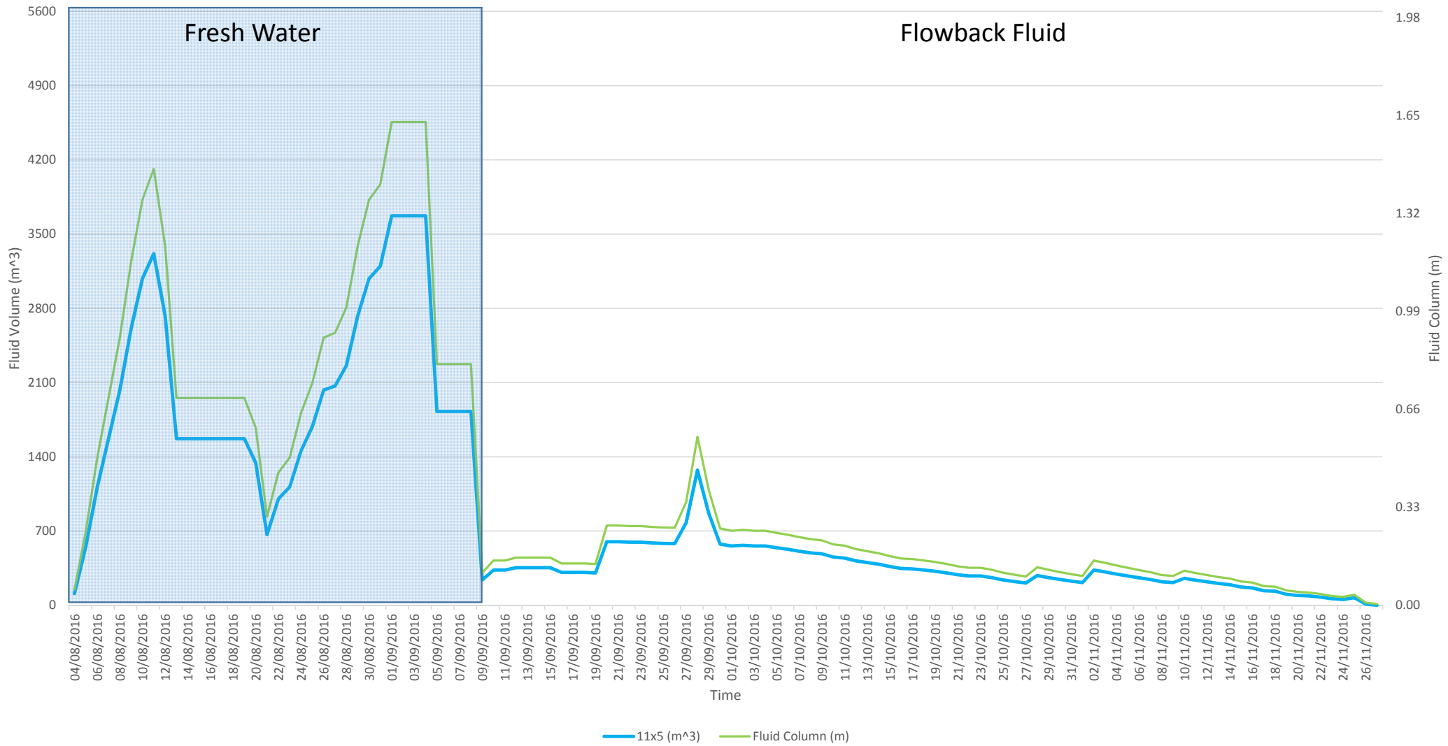
Volume and fluid column height over time Amungee NW-1 11*5 pond
